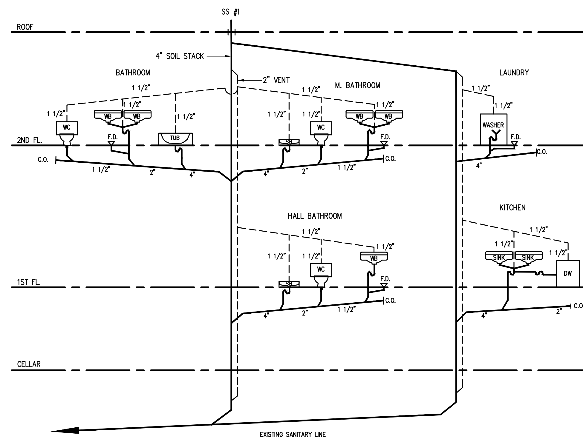
PLUMBING RISER DIAGRAM
