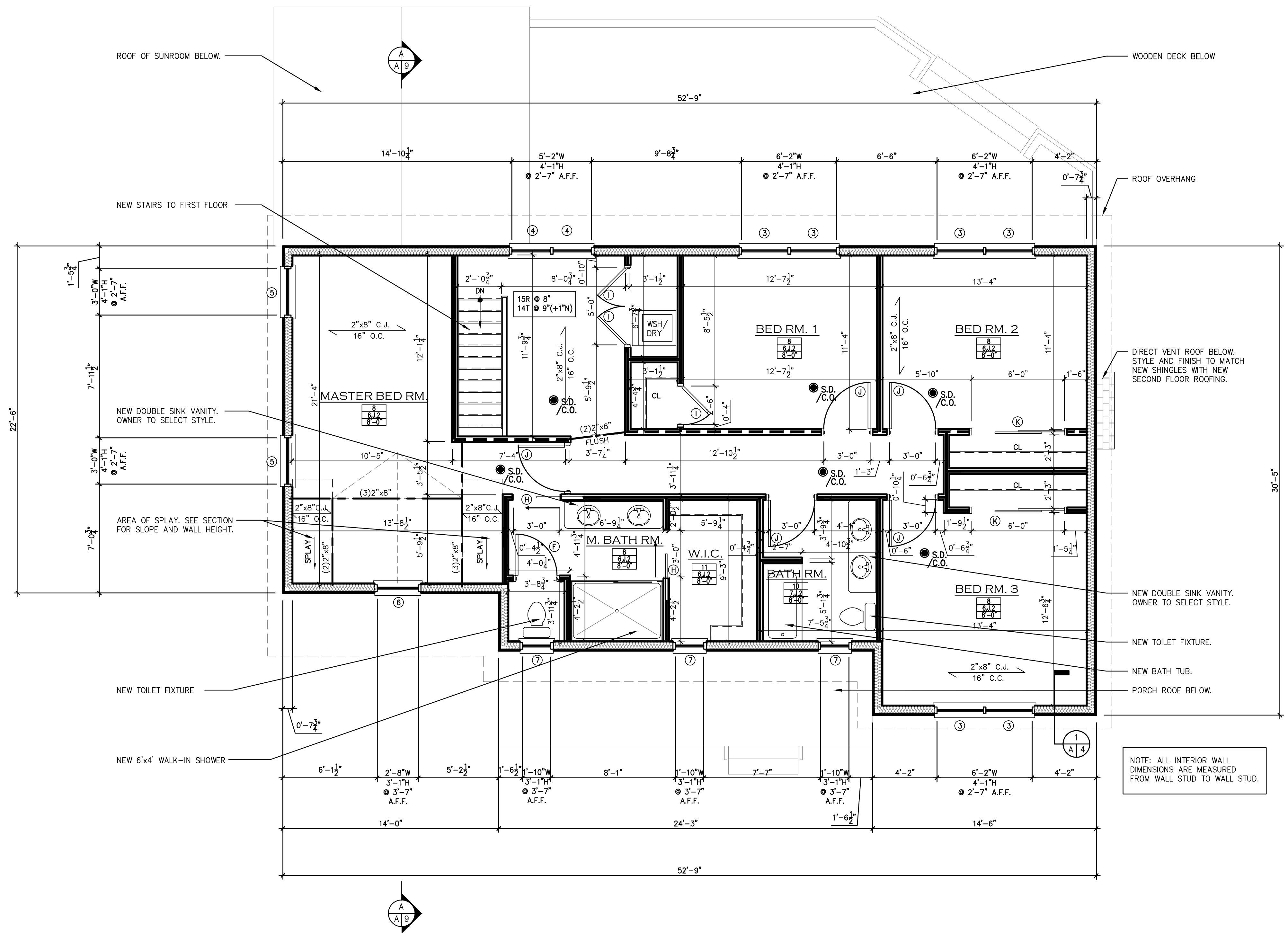
2ND FLOOR PLAN SCALE: 1/4"=1'-0"
