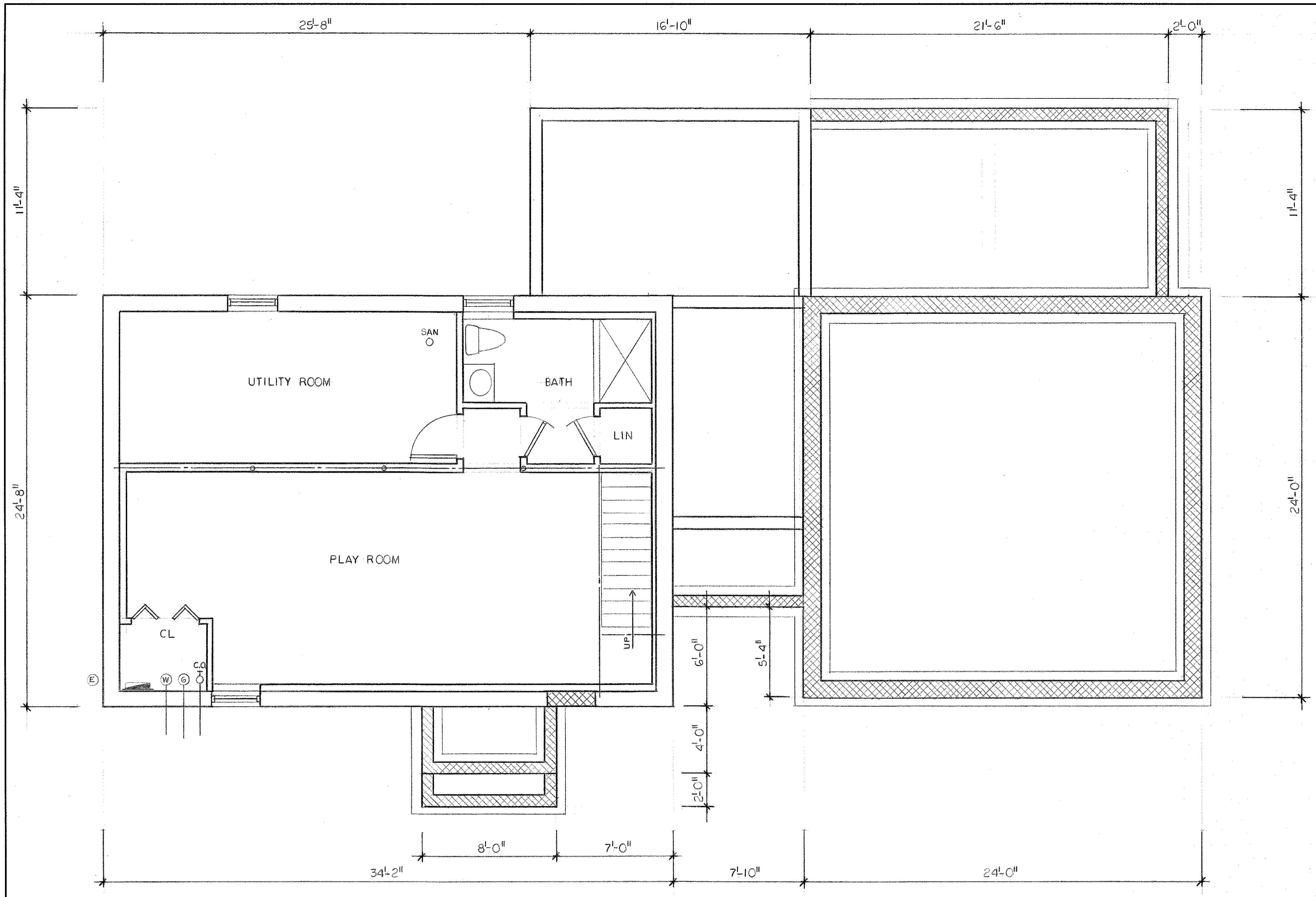
BASEMENT / FOUNDATION PLAN Scale: 1/4"=1'-0"
